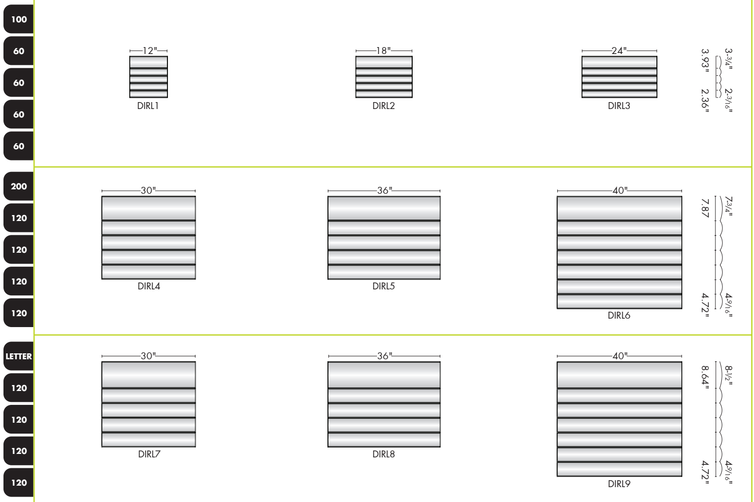
All length measurements apply to the extrusion only and exclude the end caps.
